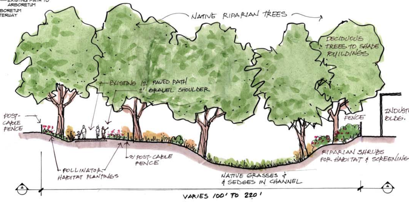
A) SECTION: BIKEWAY-RIPIARIAN CORRIDOR ON PUTAH CREEK PARKWAY
